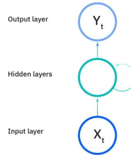
Rolled RNN
