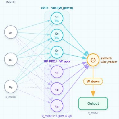
2 - Modern - 3-Layer SwiGLU
