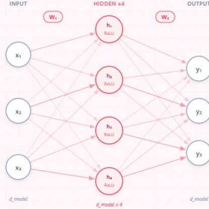
1 - Classic - 2-Layer FFN (ReLU)
