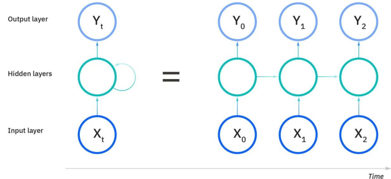
Rolled RNN
